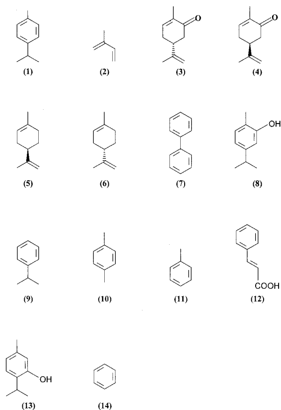
FIG. 2. Structures of compounds used in this study.
