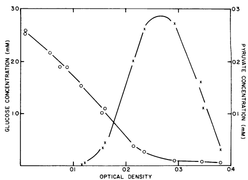
FIG. 4. Utilization of a limiting amount of glucose in HM during growth of MJ-1 (O) and appearance in and disappearance from the medium of excreted pyruvate (x).
