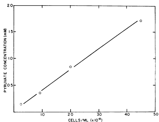
FIG. 3. Appearance of excreted pyruvate as a function of normal cell growth in HC plus glucose.
