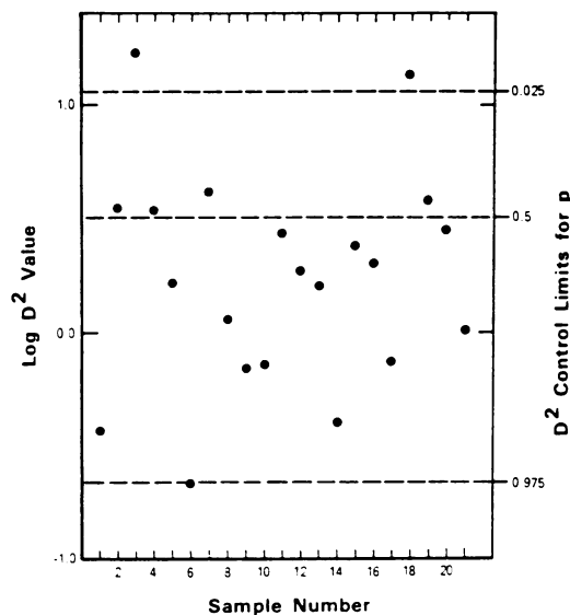
FIG. 3. D 2 analyses of 21 samples of diverse origin analyzed on YN-6 medium.
