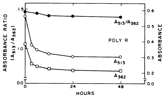
FIG. 2. A_{513} (○), A_{362} (□), and A_{513}/A_{362} ratio (●) of Poly R in culture filtrates. Cultures were 100% O_2 grown, after which they were inactivated with N_3^- , and the dye was added as described in the text. Aliquots (0.1 ml) of medium were removed at the times indicated and diluted 10-fold with water.
