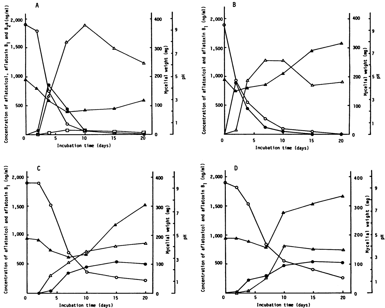
FIG. 2. Time course of fungal growth, pH of culture filtrates, and detected amount of AFL, AF-B 1 , and AF-B 2a in the cultures inoculated with four fungal strains. (A) A. niger ; (B) Rhizopus sp.; (C) A. flavus ; (D) E. herbariorum . Symbols: ○, AFL; ●, AF-B 1 ; □, AF-B 2a ; △, mycelial weight; ▲, pH. The values of mycelial weight and pH are means of two determinations, and the values of AFs and AFL are means of three determinations.
