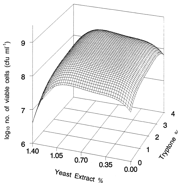
FIG. 2. Response surface for the effects of tryptone and yeast extract on the growth of L. casei at glucose = 1.58\% and temperature = 35^{\circ}\text{C} .
