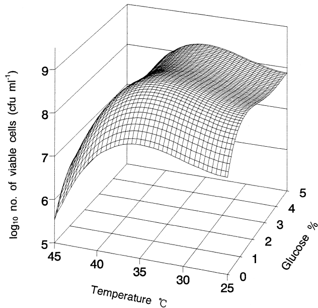
FIG. 7. Response surface for the effects of glucose and temperature on the growth of L. casei at tryptone = 3.035% and yeast extract = 0.892%.
