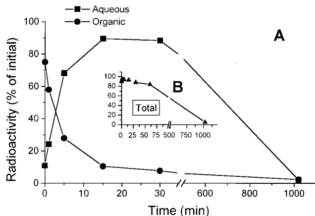
FIG. 6. [ ^{14}\text{C} ]atrazine metabolism by cell extracts prepared from Pseudomonas sp. strain ADP. The initial atrazine concentration was 100 ppm. The concentrations of atrazine and water-soluble metabolites were determined as described in Materials and Methods. (A) Time course of the disappearance of organic-soluble atrazine and appearance and disappearance of water-soluble intermediates; (B) disappearance of total ^{14}\text{C} from the incubation mixture.
