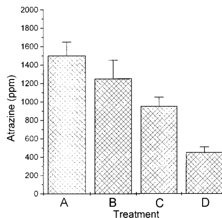
FIG. 7. Atrazine degradation in aged soil. The treatments were control, brought to 85% of water-holding capacity (A), Pseudomonas sp. strain ADP added (B), soil brought to 85% of water-holding capacity with water containing sodium citrate (C), and a combination of treatments B and C (D). The experimental details are described in Materials and Methods.
