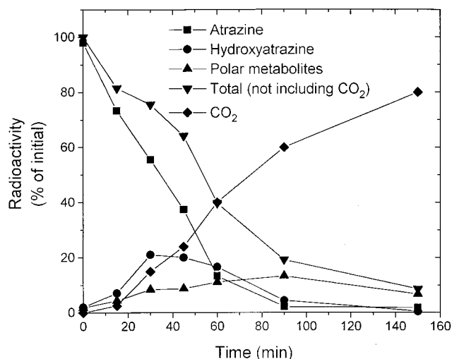
FIG. 4. Metabolism of 100 ppm of [ ^{14}\text{C} ]atrazine by resting-cell suspensions of Pseudomonas sp. strain ADP showing formation of water-soluble metabolites and, ultimately, \text{CO}_2 .
