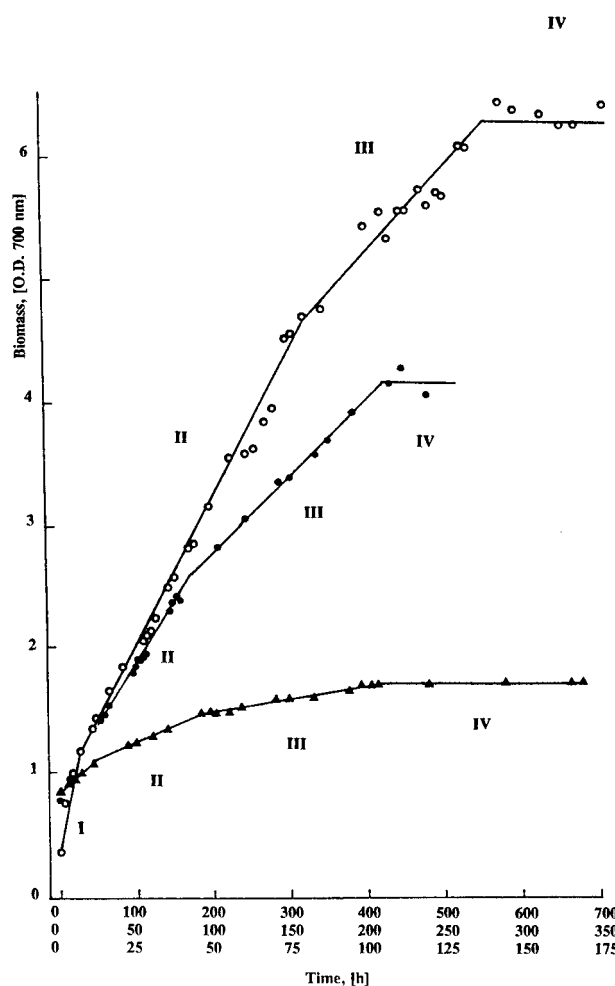
FIG. 1. Continuous cultivation on various substrates of A. eutrophus JMP 134 with 100% biomass retention. Substrates were fed at constant rates of 278 \mu mol of fructose per h ( \circ ; scale, 0 to 700 h), 430 \mu mol of phenol per h ( \bullet ; scale, 0 to 350 h), and 755 \mu mol of 2,4-D per h ( \blacktriangle ; scale, 0 to 175 h).
