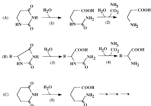
FIG. 1. Metabolic transformation pathways for dihydropyrimidine (A), hydantoin (B), and cyclic imides (C). Enzymes: 1, dihydropyrimidinase; 2, \beta -ureidodropionase; 3, hydantoinase; 4, N -carbamoyl amino acid amidohydrolase; 5, imidase.
