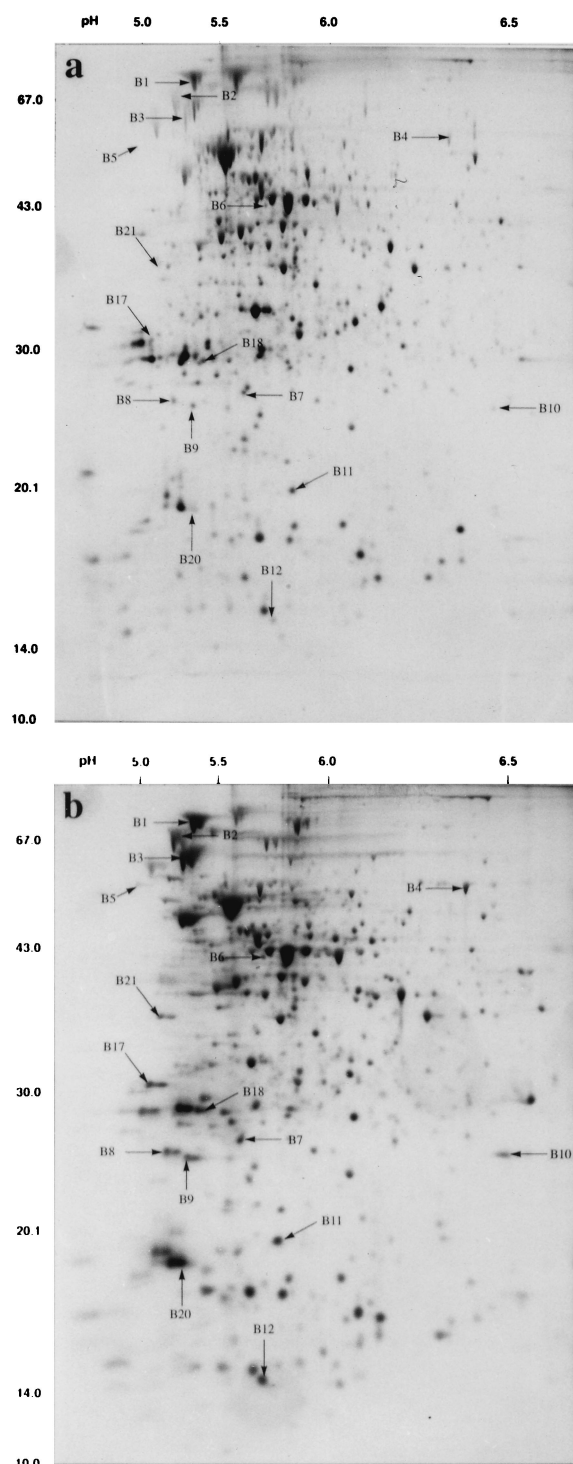
FIG. 2. Two-dimensional autoradiograms of 35 S-labeled whole cells from exponential nontreated (a) and pH 10.5-adapted (b) E. faecalis ATCC 19433. The proteins correspond to the overlap between alkaline pH and bile salts stress proteins. The DnaK and GroEL homologous proteins are indicated by B2 and B3, respectively. Equal amounts of radioactivity (approximately 250,000 cpm) were loaded onto the first-dimension gels. A uniform 14% (wt/vol) sodium dodecyl sulfate-polyacrylamide gel was used for second-dimension electrophoresis. Labeled proteins were visualized by autoradiography after 7 months of exposure. M s (in thousands) are indicated to the left of each gel.
