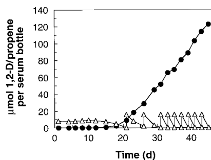
FIG. 2. Reductive dechlorination of 1,2-D (triangles) to propene (circles) in sediment-free, nonmethanogenic cultures. Acetate (10 mM) and \text{H}_2 (8 ml) were supplied as potential electron donors. 1,2-D was respiked when depleted, and \text{H}_2 was fed when the concentration was below 500 ppmv. Data are the mean values for duplicate cultures.
