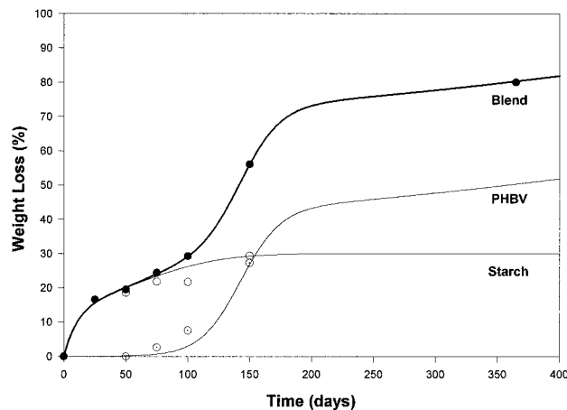
FIG. 4. Computed polymer weight loss profiles (curves) for a 30% starch-70% PHBV blend. Data are from station 2. Symbols: ●, total weight loss for test specimens; ○ and ⊙, experimental weight loss for individual starch (○) and PHBV (⊙) polymers obtained by dichloromethane extraction of test specimens, plotted after the starch and PHBV curves were determined with the mathematical model.
