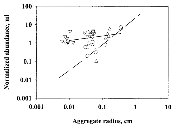
FIG. 11. Steady-state abundances of bacteria on aggregates as a function of aggregate size predicted from equation 13 (dashed line) compared to actually observed abundances on field-collected aggregates (symbols and solid line) (taken from the compilation of Kiørboe [22]). The different symbols refer to data from different studies. The predicted relation assumes a bacterial diffusivity of 10^{-5} \text{ cm}^2 \text{ s}^{-1} . Abundances have been normalized by ambient concentrations of bacteria. The predicted abundance increases with aggregate size raised to a power of 1.45 within the aggregate size range considered, while the log-log regression for the field-collected aggregates has a slope of 0.25.
