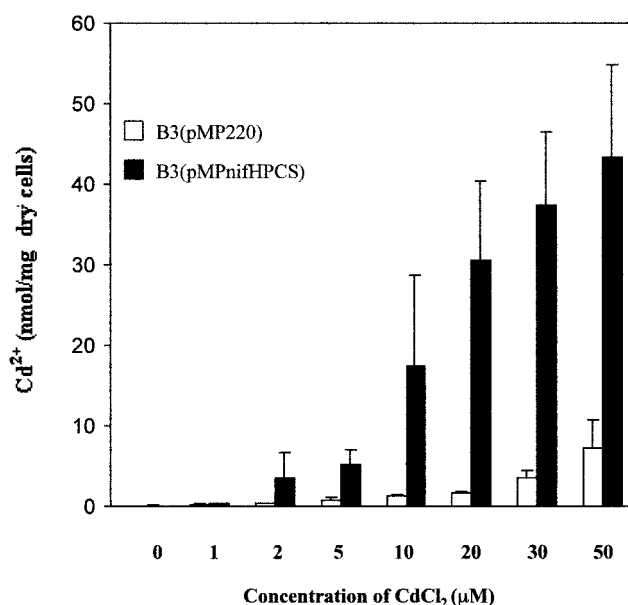
FIG. 4. Effects of CdCl 2 on the synthesis of PCs in M. huakuii subsp. rengei B3. Determinations were made by atomic absorption spectrometry of the amount of Cd 2+ accumulated in strain B3 that harbored the empty vector, namely, B3(pMP220) cells, and in B3 cells that contained the PCS At gene, namely, B3(pMPnifHPCS) cells. The amount of Cd 2+ bound to bacterial cells is indicated in nanomoles per milligram (dry weight) of cells. The values shown are means ( \pm standard deviations) of the results for three independent experiments in each case. Bacteria were grown under microaerobic conditions in the presence of various concentrations of CdCl 2 (1 to 50 \mu M) as indicated for 40 h.
