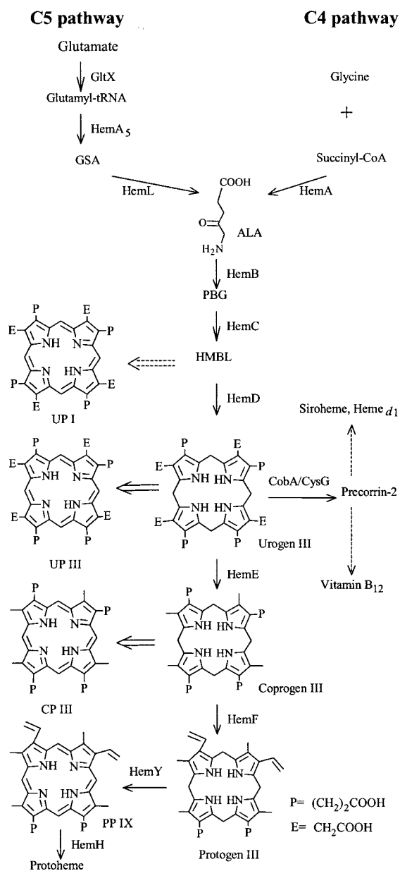
FIG. 1. Overview of the biosynthesis of tetrapyrroles with gene products indicated. Dashed lines denote multistep pathways, and broad arrows indicate nonenzymic steps.
