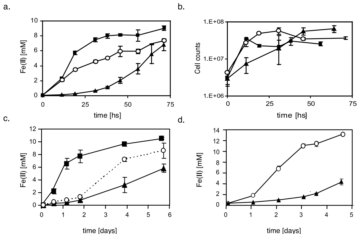
FIG. 4. Total Fe(II) produced (a) and cell growth achieved (b) by the reduction of poorly crystalline iron (hydr)oxide by S. oneidensis MR1 in the absence (▲) or presence of 10 \mu M AQDS (■) or 10 \mu M PCN (○). (c) Total Fe(II) produced by the reduction of poorly crystalline iron (hydr)oxide by S. oneidensis MR1 in the absence (▲) or presence of a final 1:10 dilution of filtered culture supernatant from the WT strain PCL1391 (■) or the mutant PCL1119 (○). (d) Total Fe(II) produced by the reduction of poorly crystalline iron (hydr)oxide by S. oneidensis MR1 in the absence (▲) or presence (○) of 15 to 20 \mu M bleomycin. Data represent the average value of duplicate experiments, with bars showing the data range.
