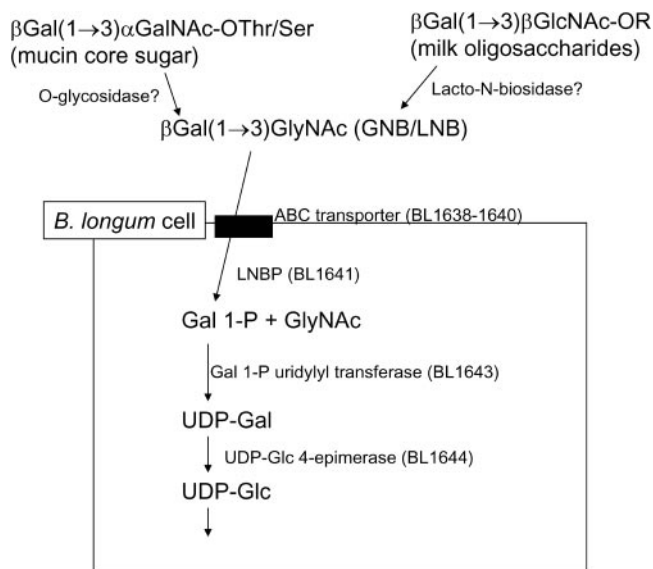
FIG. 3. Proposed scheme of lacto- N -biose metabolism.
