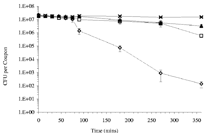
FIG. 4. Effect on E. coli O157 viability of a 6-h exposure to either stainless steel (×), C873000 (◇), C83600 (▲), or C83300 (□) at 4°C in the presence of liquid beef extract. Coupons (1 cm by 1 cm) were inoculated with 20 \mu l of a 19-h E. coli O157 culture mixed with liquid beef extract (25%). Following the exposure period, coupons were transferred to tubes containing 10 ml sterile PBS with 2-mm-diameter glass beads. Cells were subsequently removed from the coupons into suspension by vortexing, and 100 \mu l was removed and serially diluted to 10^{-4} in sterile PBS. TSB plates were then inoculated (50 \mu l) for each dilution and subsequently incubated at 37°C for 18 h. Postincubation, the number of CFU on each plate was counted and used to calculate the number of viable CFU per coupon. Points represent the means ( n = 3 ) \pm SEM.
