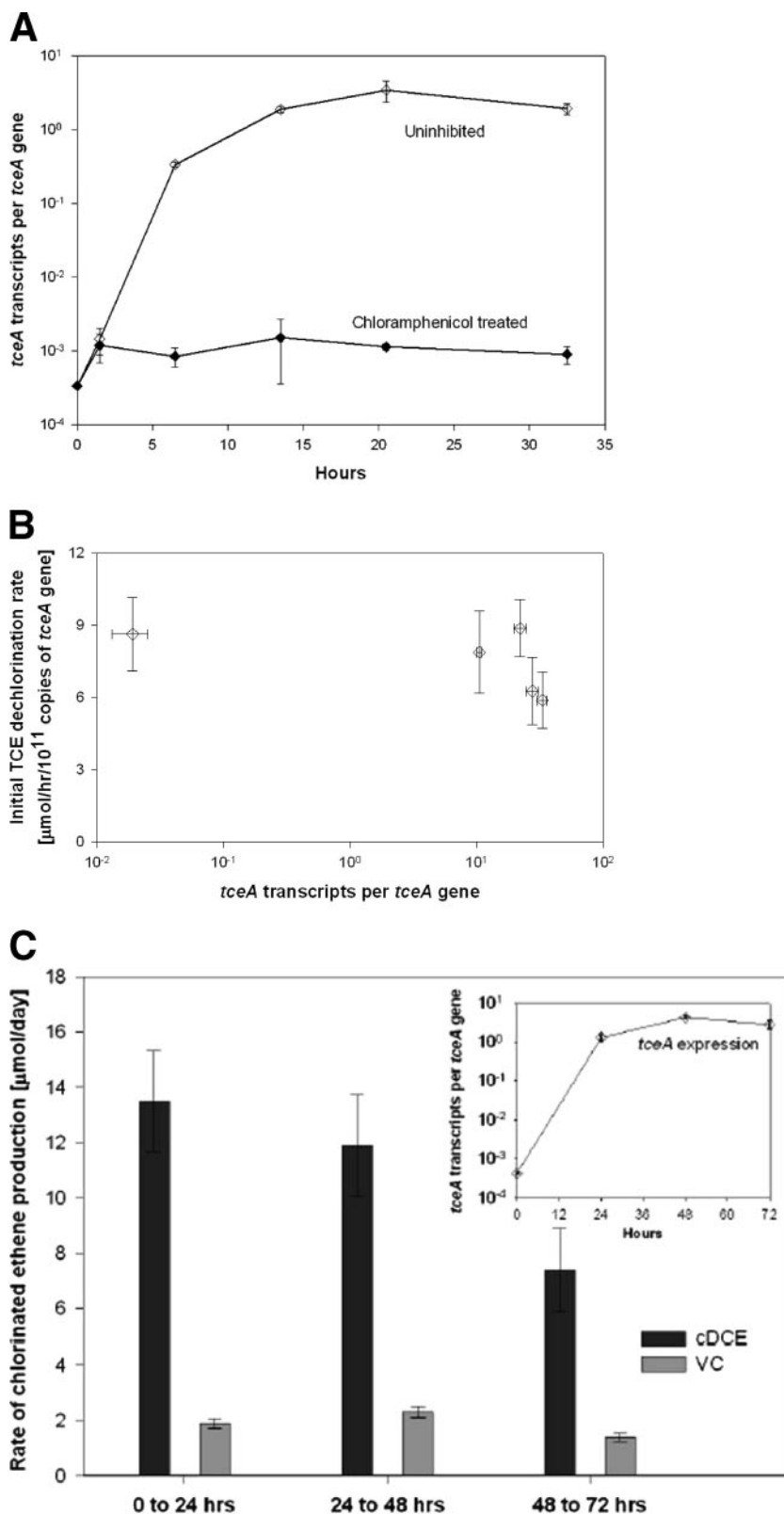
FIG. 4. (A) tceA gene expression profile with and without the influence of chloramphenicol. (B) Initial dechlorination rate of TCE in the presence of chloramphenicol after the establishment of different transcript levels in five respective cultures. Rate measurements are normalized to the tceA gene copy number. The error bars for the rate measurement represent the 95% confidence interval of the slope of TCE dechlorination over 10 h. (C) Dechlorination activity of the ANAS enrichment culture over three consecutive days as represented by the rate of production of the TCE daughter products cDCE and VC every 24 h. Error bars represent the 95% confidence interval. The inset graph shows tceA gene expression during the 3 days of active dechlorination.
