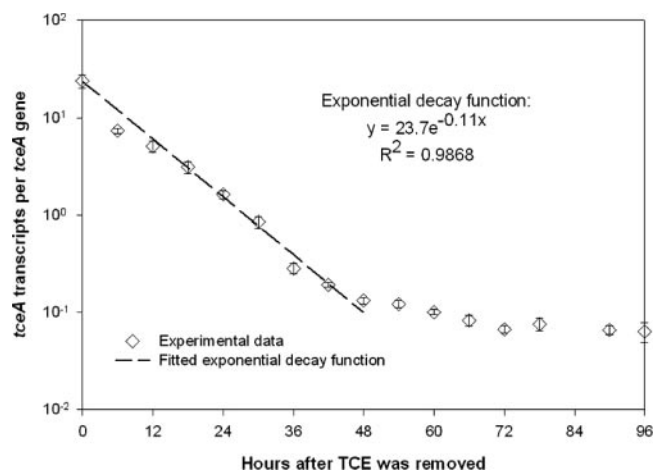
FIG. 3. Decay profile of tceA transcripts when chlorinated ethenes were stripped from the culture after 24 h of active dechlorination.
