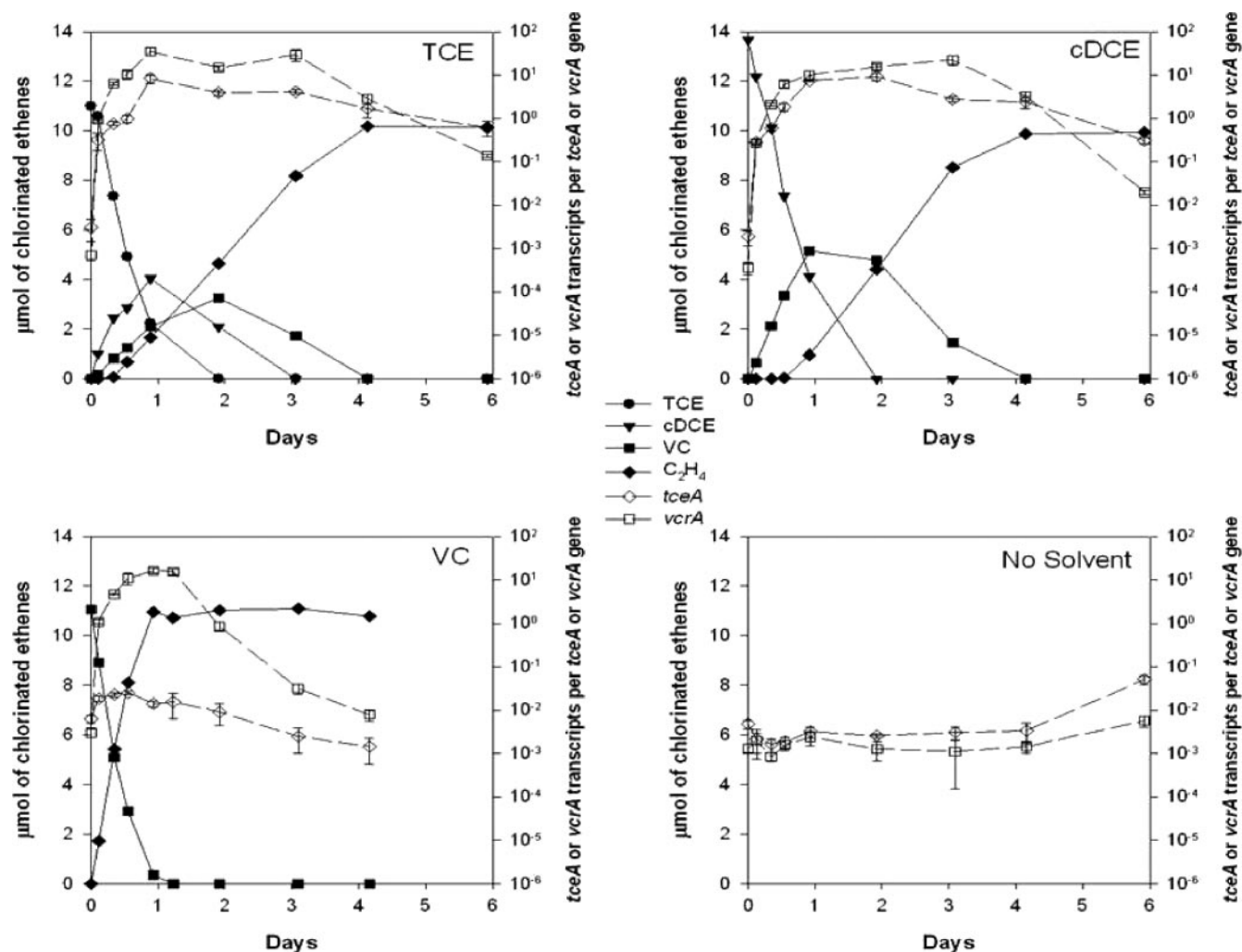
FIG. 2. Reductive dechlorination of chlorinated ethenes (solid lines) and expression profile of the tceA and vcrA genes (dashed lines) over a feeding cycle for ANAS. Expression measurements are calculated from averages of triplicate qPCRs and RT-qPCRs, and error bars represent 1 standard deviation.
