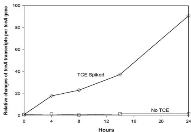
FIG. 1. tceA gene expression profile of a pure culture of Dehalococcoides ethenogenes 195 in the presence and absence of TCE over 24 h. Measurements of tceA transcripts per tceA gene at each time point are normalized to the value at time zero to obtain the relative changes. Data are calculated from averages of triplicate qPCRs and RT-qPCRs, and error bars are smaller than the box symbol.
