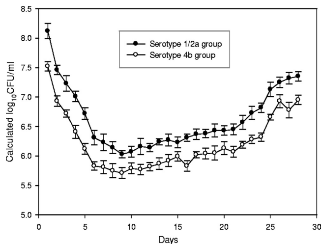
FIG. 3. Planktonic cell density of L. monocytogenes serotype 1/2a and 4b strains in diluted medium (TSBYE/10) in the group for serotype mix biofilms at the end of each 8-h incubation period in each 24-h cycle of the SFP system. The filled symbols represent serotype 1/2a strains; the open symbols represent serotype 4b strains. The error bars represent the mean and standard deviation ( n = 3 ).
